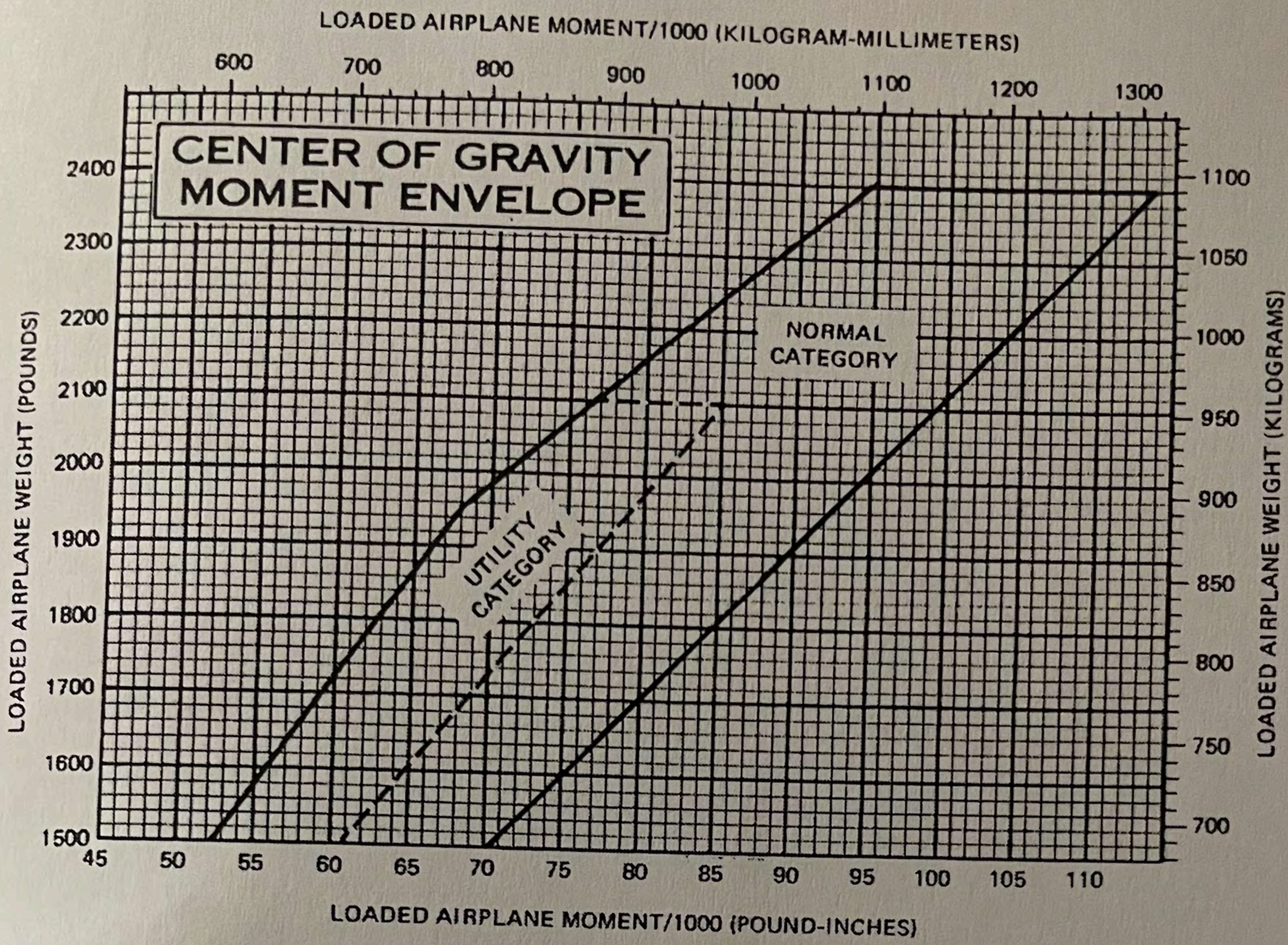
Figure 6-7. Center of Gravity Moment Envelope
