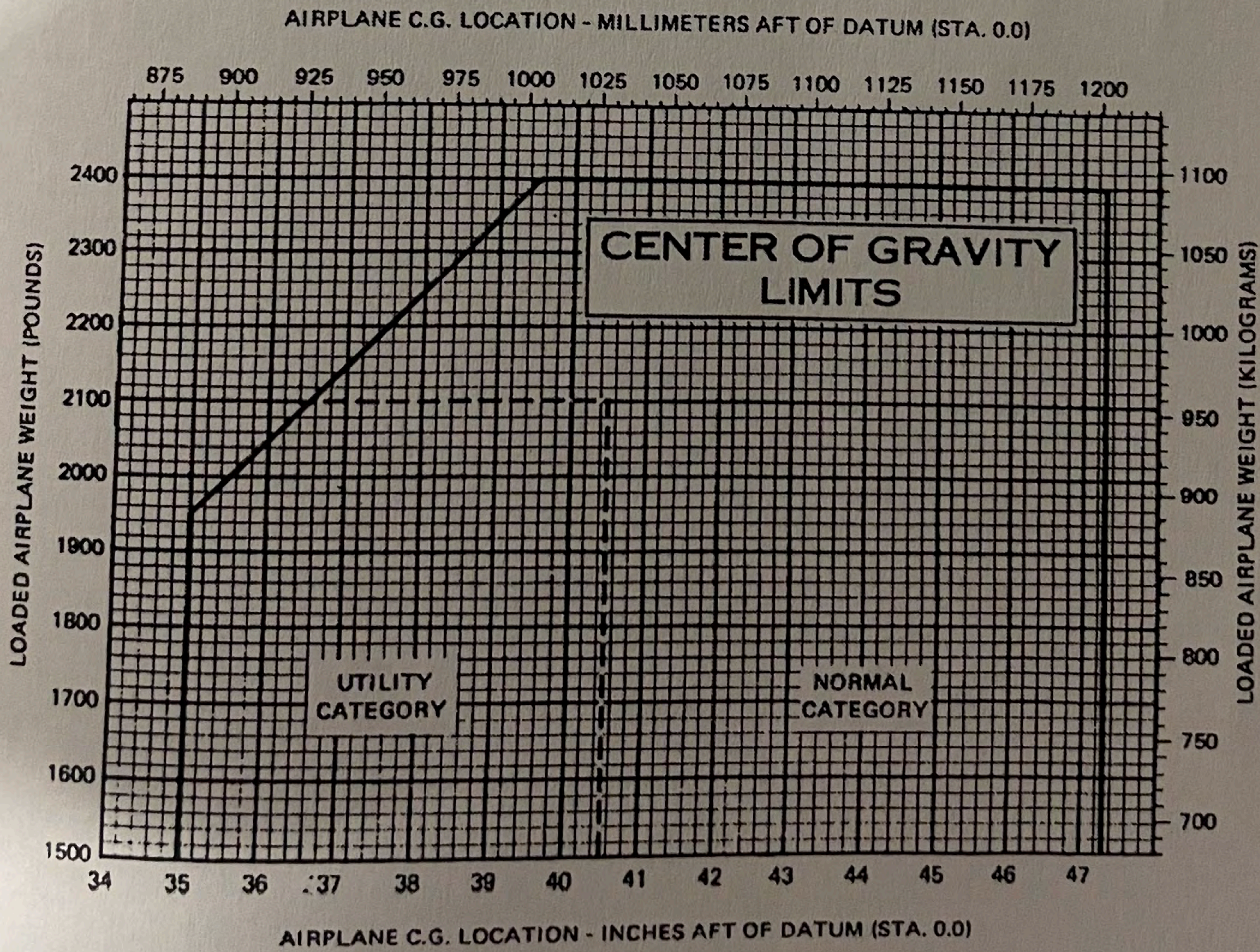
Figure 6-8. Center of Gravity Limits
